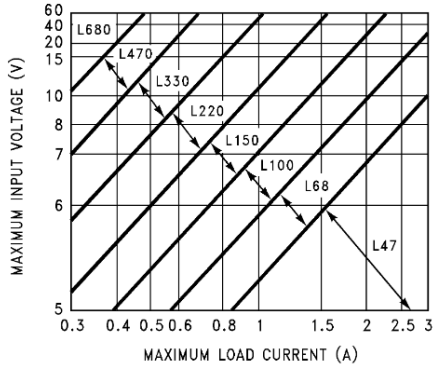
Figure 23. LM2576(HV)-3.3
