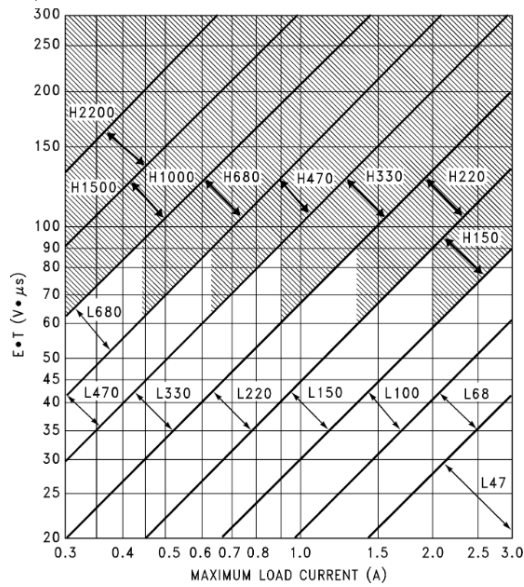
Figure 27. LM2576(HV)-ADJ
