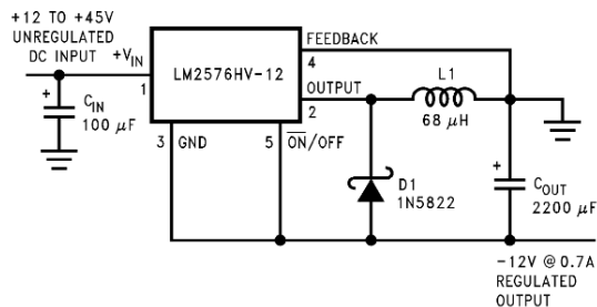
Figure 28. Inverting Buck-Boost Develops -12V
