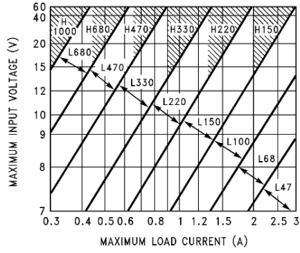
Figure 24. LM2576(HV)-5.0
