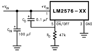
Figure 32. Delayed Startup
