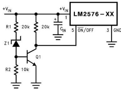
Figure 30. Undervoltage Lockout for Buck Circuit
