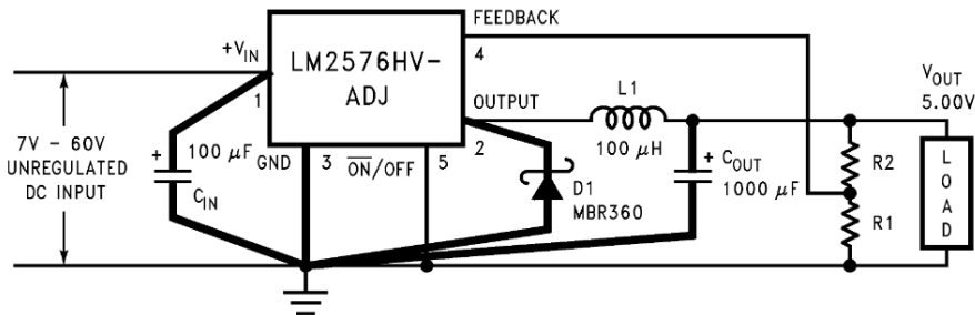
Figure 21. Fixed Output Voltage Versions
