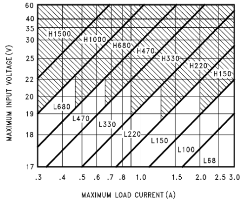
Figure 26. LM2576(HV)-15
