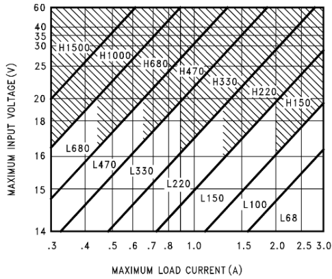
Figure 25. LM2576(HV)-12
