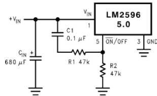
Figure 33. Delayed Startup
