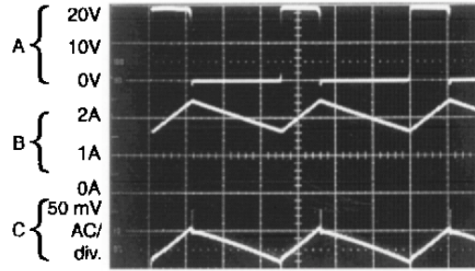
Figure 16. Horizontal Time Base: 2 \mu s /div.
