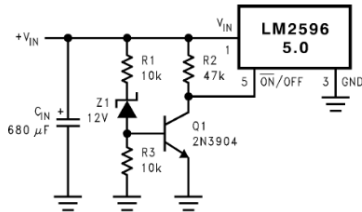
Figure 34. Undervoltage Lockout for Buck Regulator
