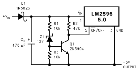
Figure 36. Undervoltage Lockout with Hysteresis for Inverting Regulator
