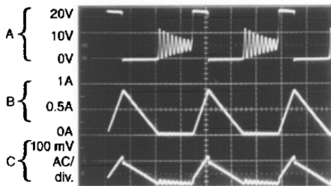
Figure 17. Horizontal Time Base: 2 \mu s /div.
