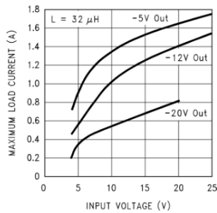
Figure 38. Inverting Regulator Typical Load Current
