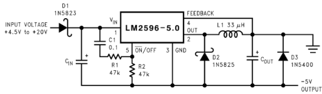
Figure 37. Inverting -5V Regulator with Delayed Startup
