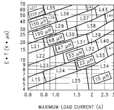
Figure 24. LM2596-ADJ
