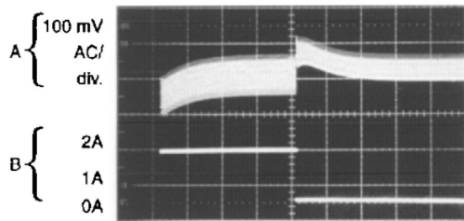
Figure 19. Horizontal Time Base: 200 \mu s /div.
