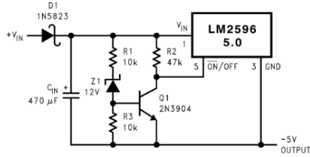
Figure 35. Undervoltage Lockout for Inverting Regulator
