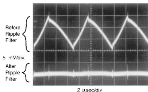
Figure 29. Post Ripple Filter Waveform
