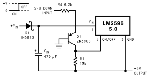
Figure 39. Inverting Regulator Ground Referenced Shutdown
