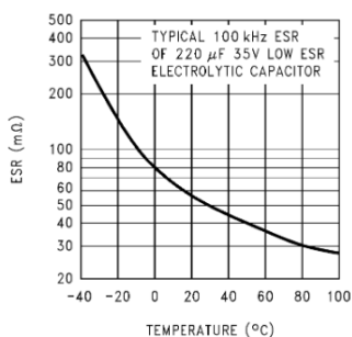
Figure 27. Capacitor ESR Change vs Temperature
