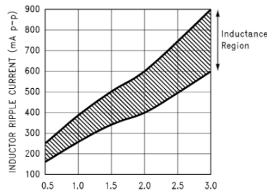
Figure 30. Peak-to-Peak Inductor Ripple Current vs Load Current
