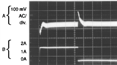
Figure 18. Horizontal Time Base: 100 \mu s /div.
