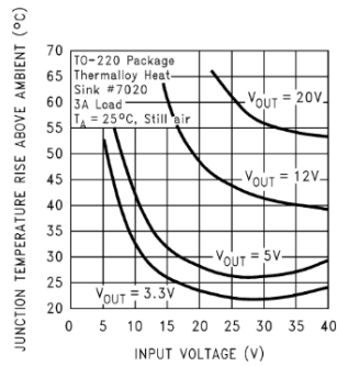
Circuit Data for Temperature Rise Curve
